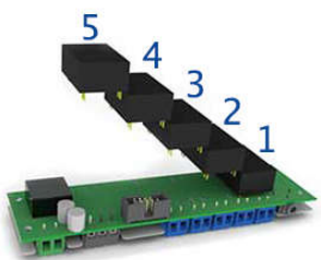
DC LED Drivers for Channels 1-5
