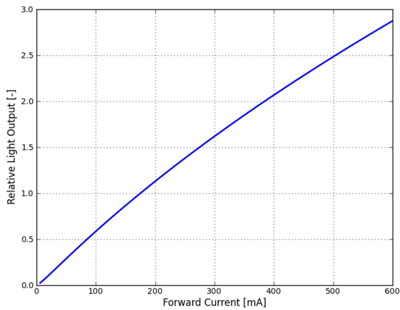
Figure 20. Typical relative luminous flux vs. forward current for LUXEON K (LXXx-PWxx-0206) with multi-junction die.
