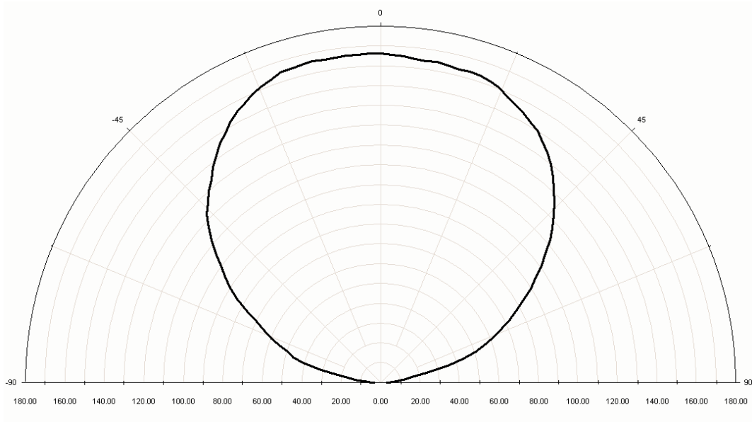
Figure 15: Typical Polar Radiation Pattern for White Lambertian.
